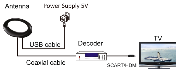
Pic. 2 Connection by using the antenna power supply
